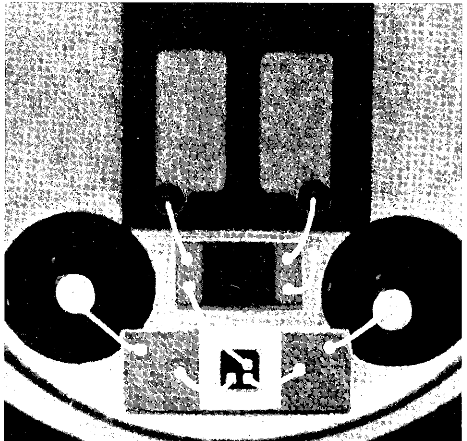
Figure 11. Header of dual element, series opposed lithium tantalate detector with load resistor and FET. Bottom electrode unconnected (floating). Wire from resistor to header makes case ground. Photo retouched to make 0.025mm (1 mil) gold wire visible.
