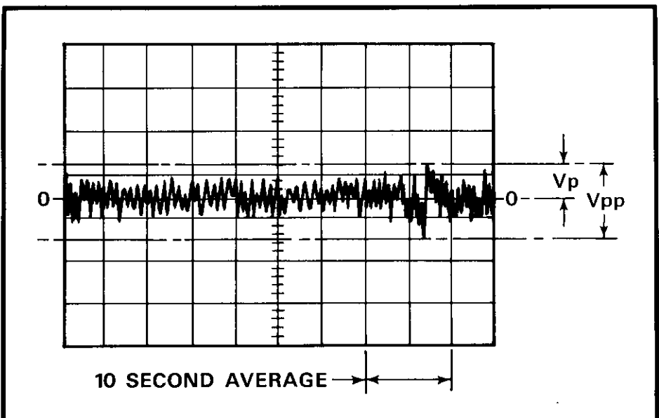
Figure 8. Peak-to-peak noise determination.
