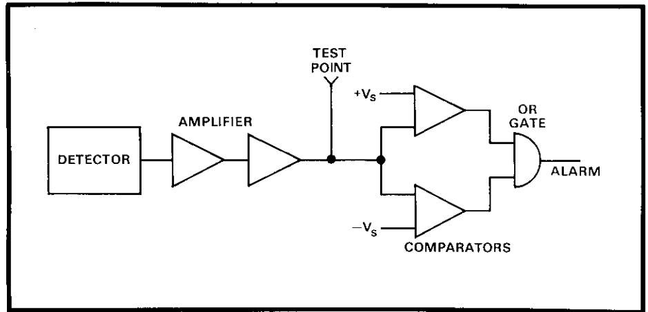
Figure 7. Noise measuring test setup.
